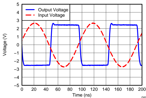
Figure 25. Comparator Response to Input Voltage (No Phase Inversion)
