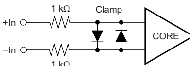
Figure 26. TLV3201 equivalent input structure
